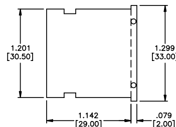
DPS910A2 Spacer
